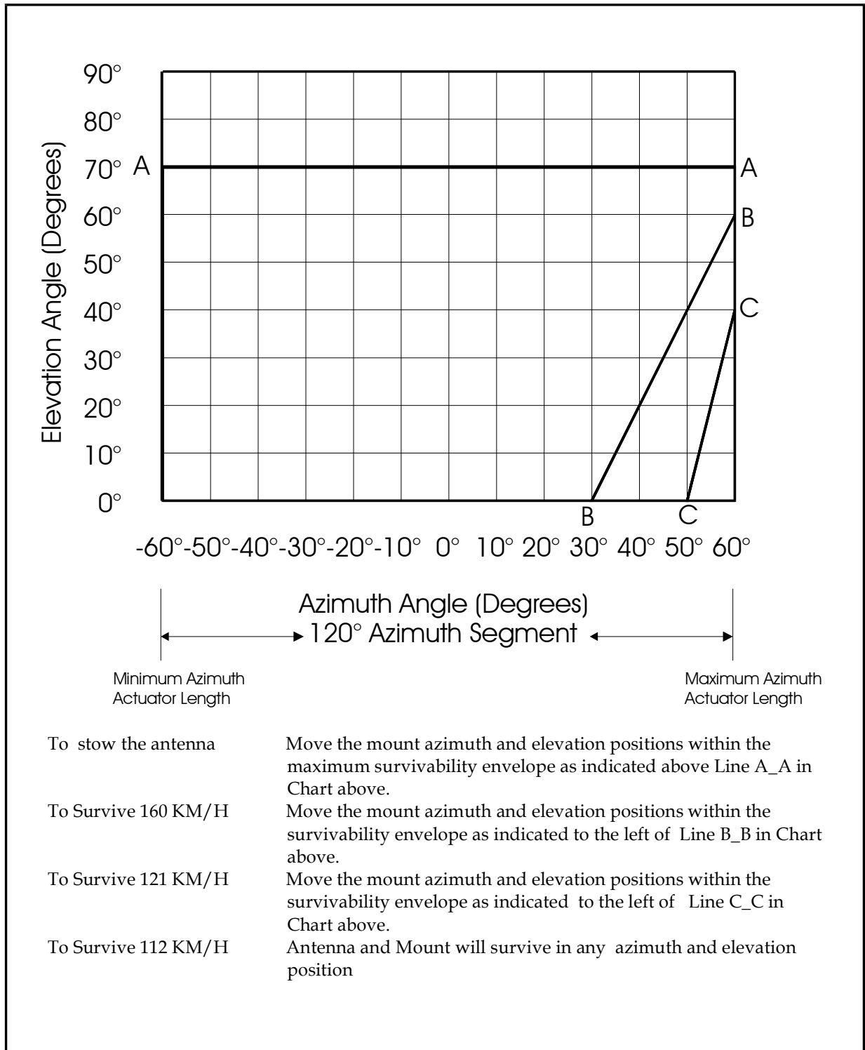
Figure 1-2. Elevation and Azimuth Angle Stow Chart for High Wind Conditions
