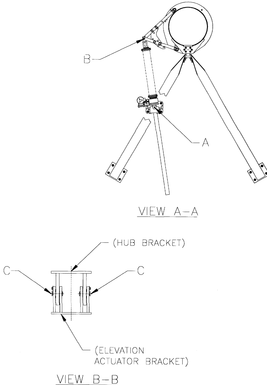
Figure 4-1. Lubrication Points (Sheet 2 of 2)
